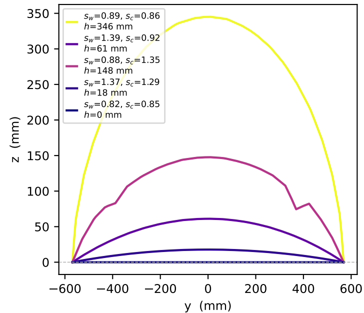
YZ cross-sections — motif2 cable
