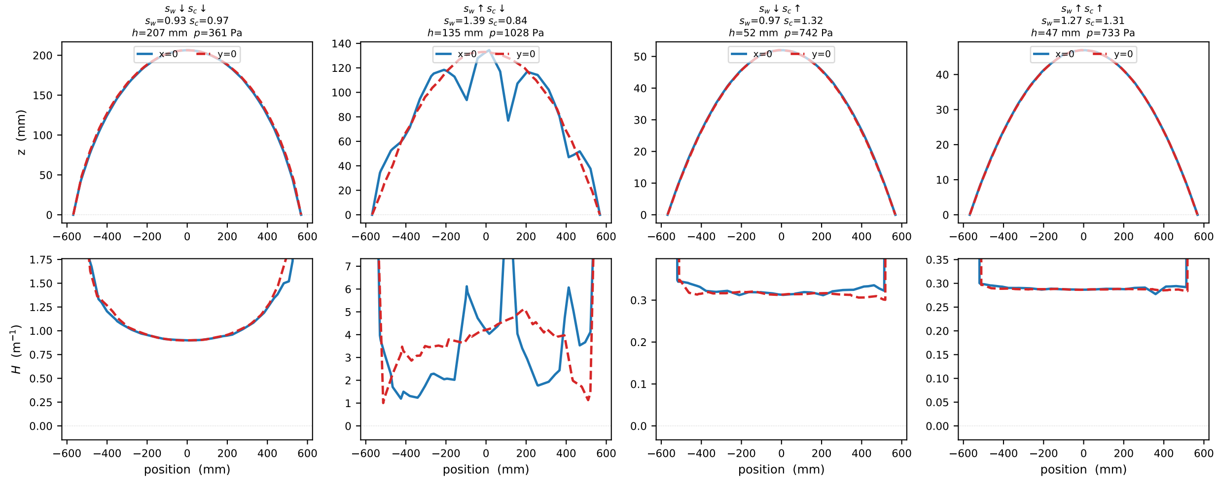
Cross-section profiles along x=0 and y=0 planes — motif1 cable (solid = x=0 , dashed = y=0 ; anisotropy visible when profiles differ)
