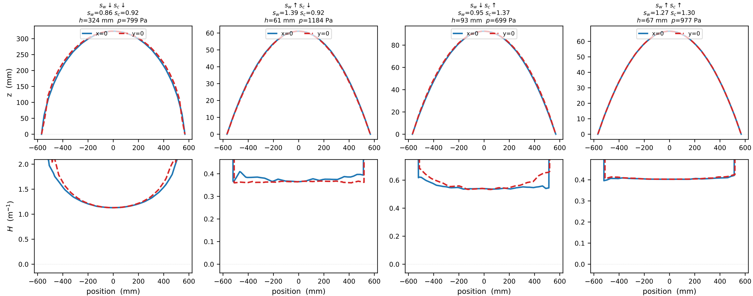
Cross-section profiles along x=0 and y=0 planes — motif2 cable (solid = x=0 , dashed = y=0 ; anisotropy visible when profiles differ)
