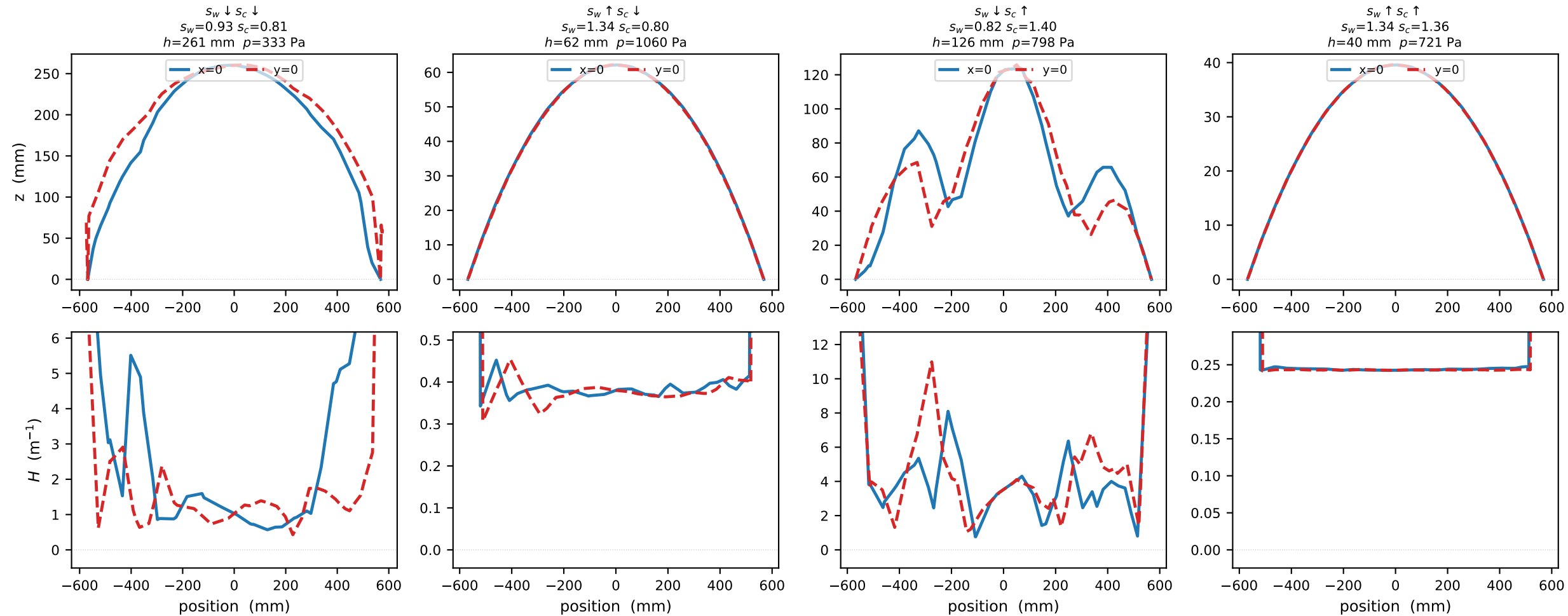
Cross-section profiles along x=0 and y=0 planes — motif2 nocable (solid = x=0 , dashed = y=0 ; anisotropy visible when profiles differ)
