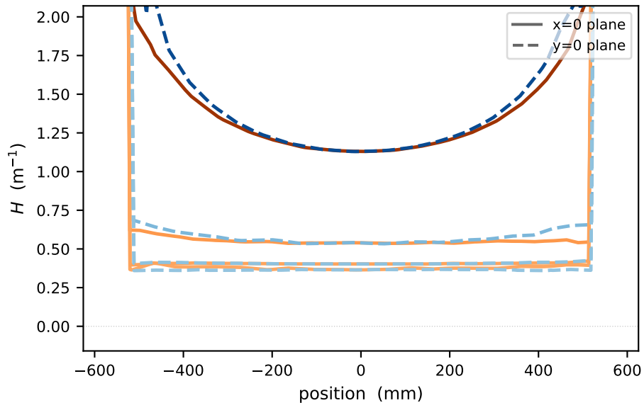
Mean-curvature profiles H(s)
