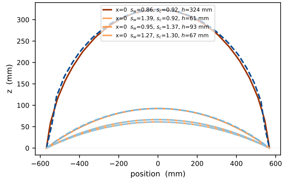
Shape profiles z(s)
