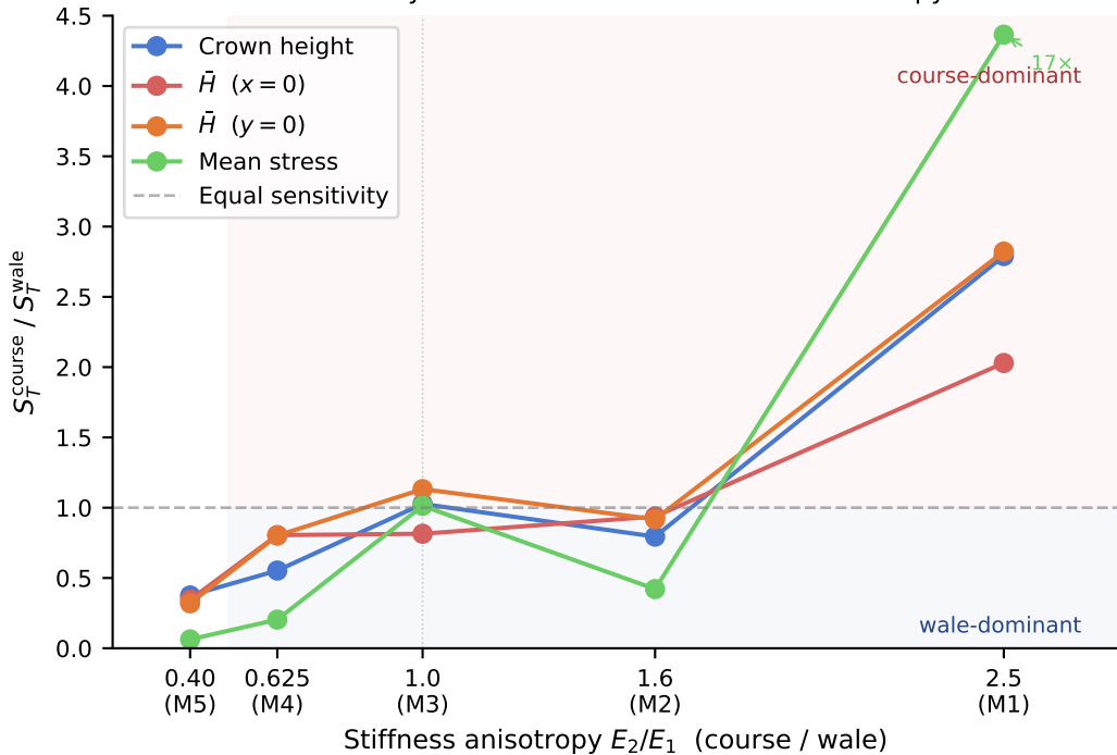
Sensitivity dominance ratio vs material anisotropy
