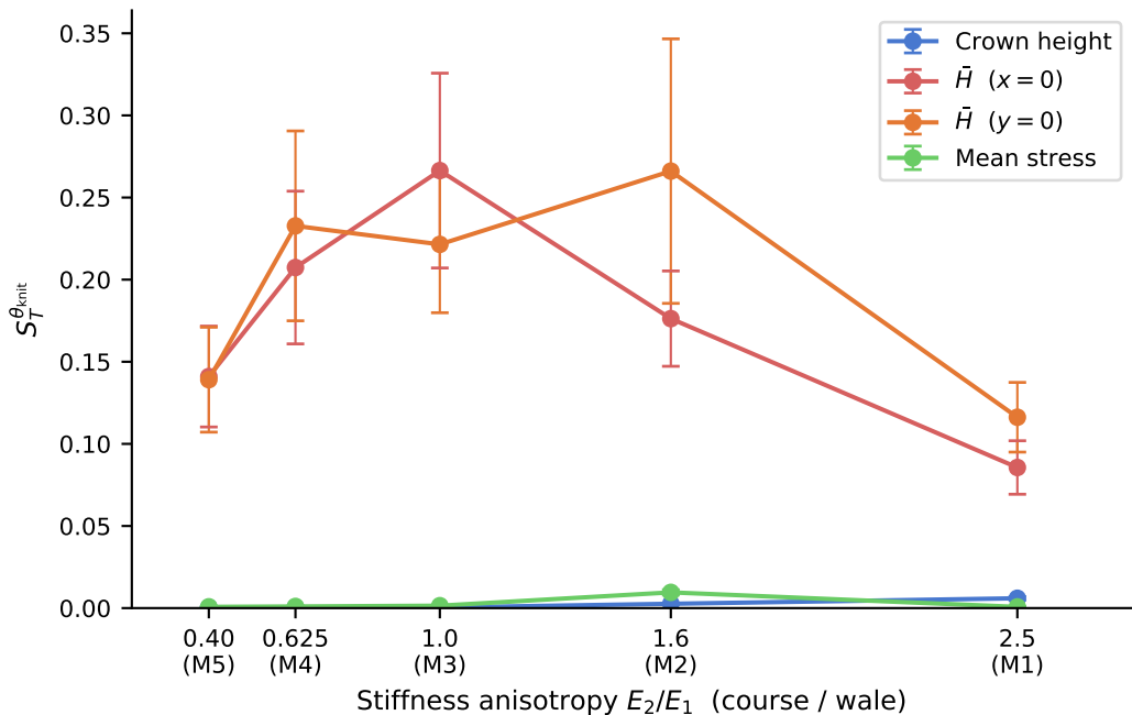
Knitting direction sensitivity vs material anisotropy
