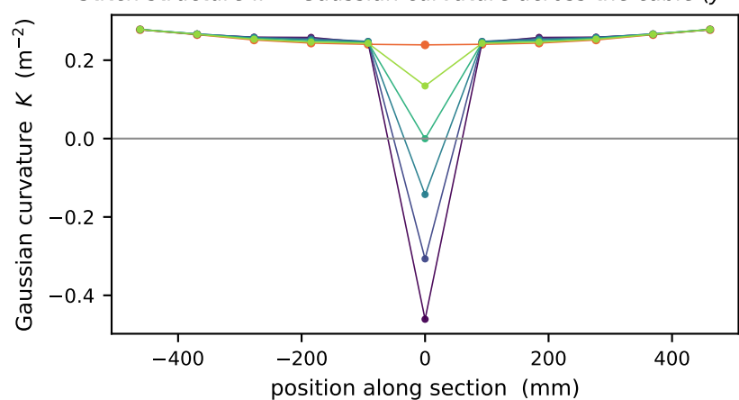
Stitch structure II — Gaussian curvature across the cable ( y=0 )
