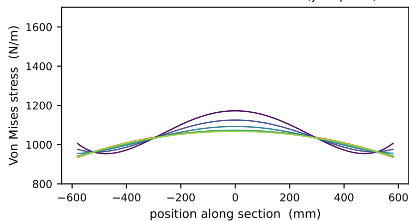
Stitch structure II — section stress ( y=0 plane)
