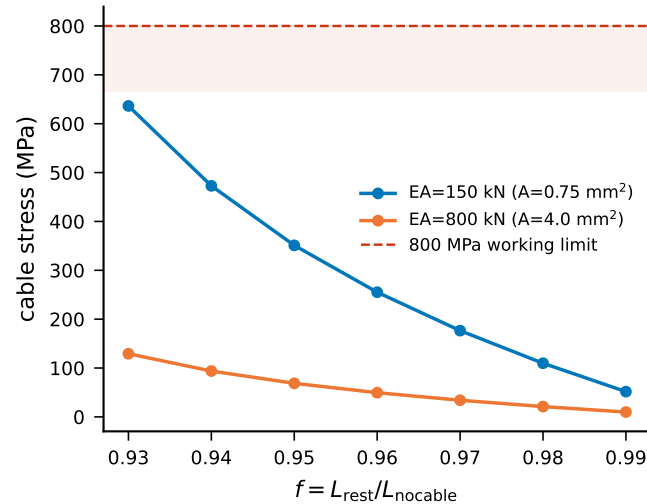
(c) cable stress (MPa)
