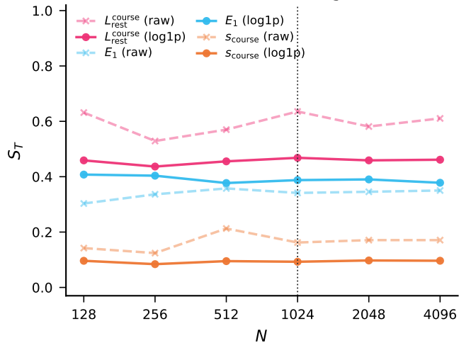
(b) T_{\text{course}}(N) : raw vs \log(1 + T)
