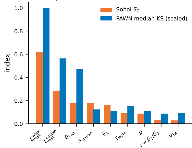
(c) cable \Delta H : variance-based vs moment-independent Spearman rank correlation 0.90
