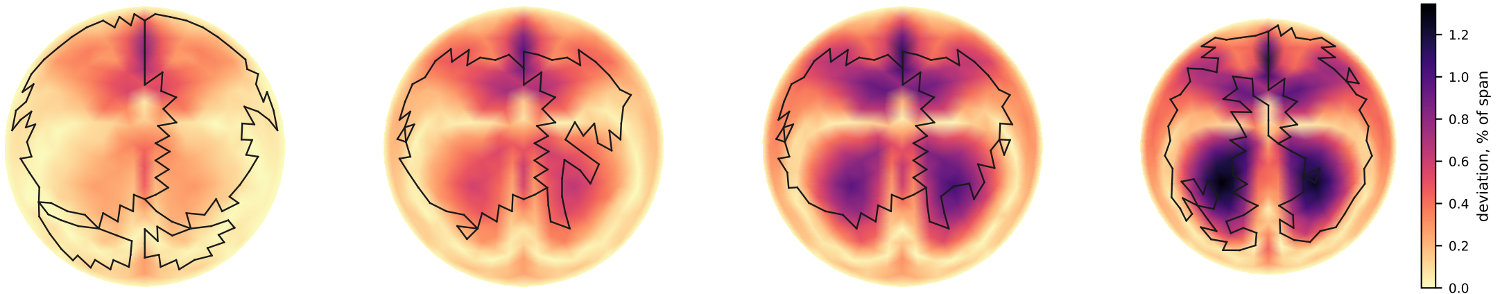
(e) strategy E: where the deviation is, each normalised by its own span; black lines are the region boundaries
