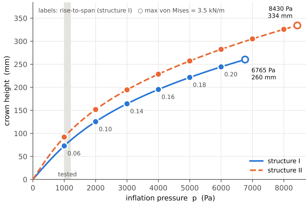
(a) crown height to the 3.5 kN/m stress limit, s_{wale} = 1.1 , s_{course} = 1.1
