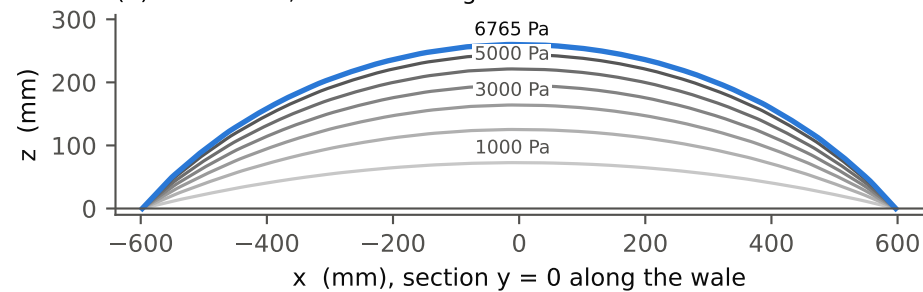
(b) structure I, section through the crown
