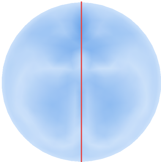
(E) Three regions, crease cable mean 2.75 mm (0.23%), max 11.8 mm (0.98%)
