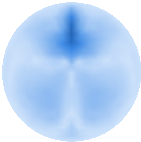
(C) Anisotropic pre-strain, no cable mean 3.35 mm (0.28%), max 24.0 mm (2.00%)
