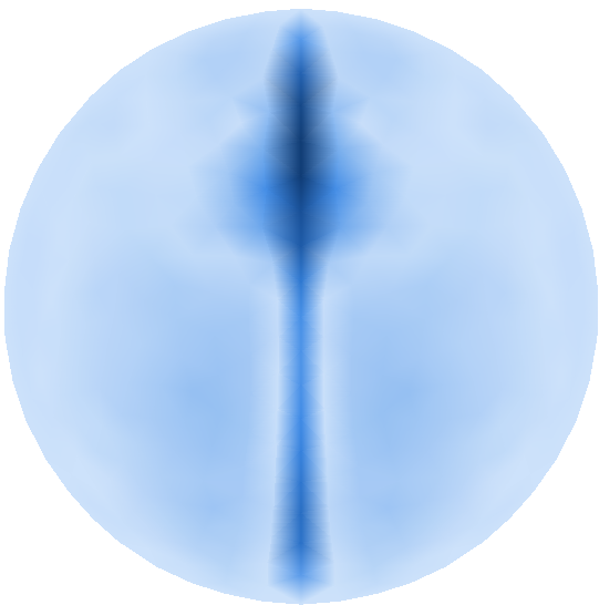
(A) Isotropic pre-strain, no cable mean 3.01 mm (0.25%), max 33.7 mm (2.81%)
