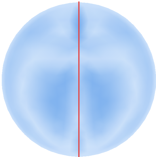
(B) Isotropic pre-strain, crease cable mean 3.01 mm (0.25%), max 10.4 mm (0.87%)
