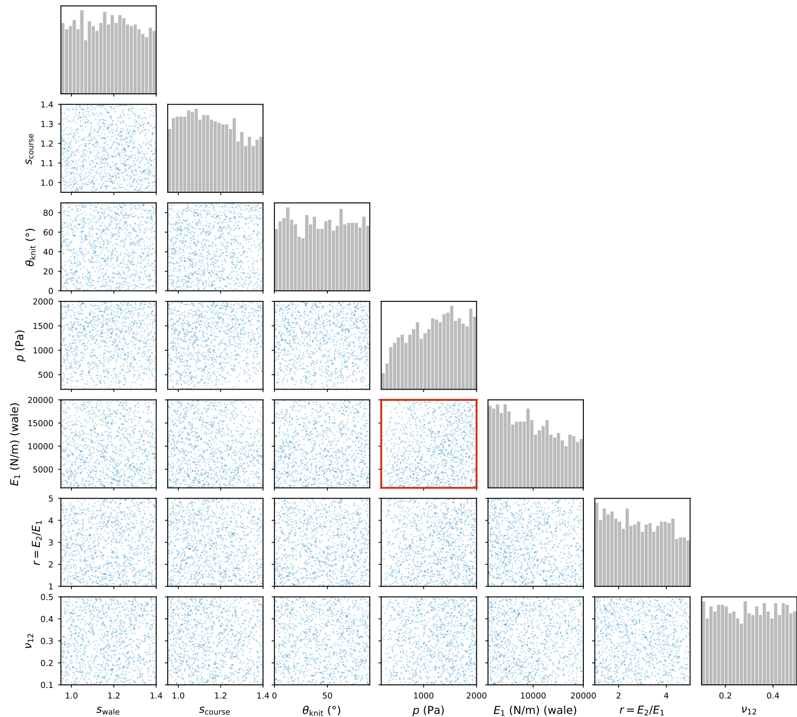
Training design coverage — no cable, validity box, s \geq 0.95 (7-D, 1095 runs of 1345 planned, 81% retained) largest pairwise |r| = 0.152 (pressure, E1), outlined in red
