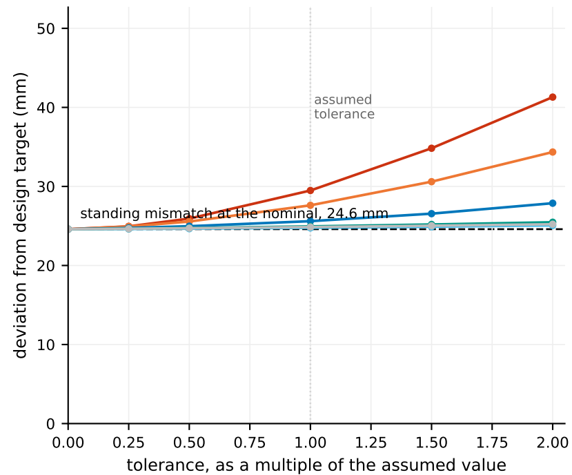
(c) creased shell: deviation from the design target
