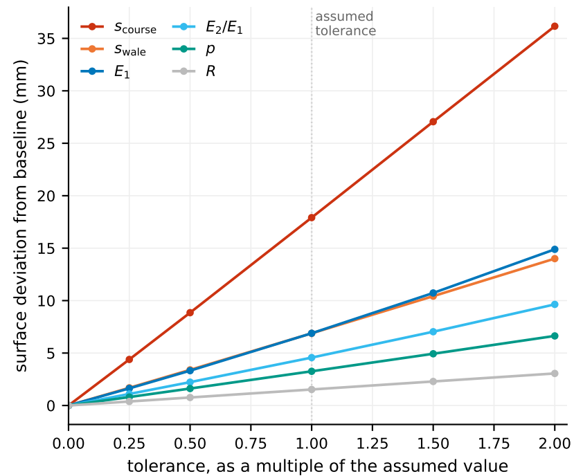
(a) circular dome: how far the surface moves
