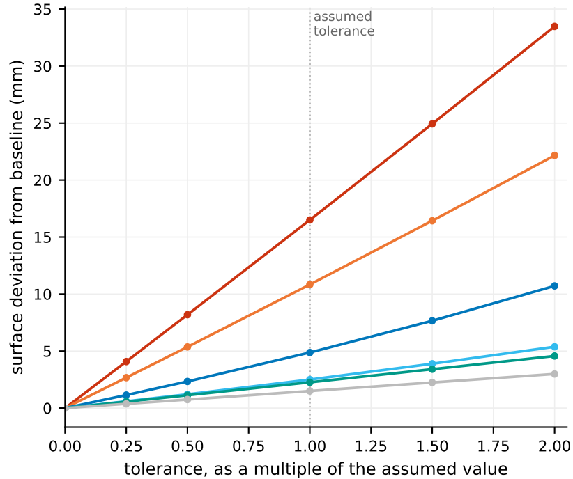
(b) creased shell: how far the surface moves
