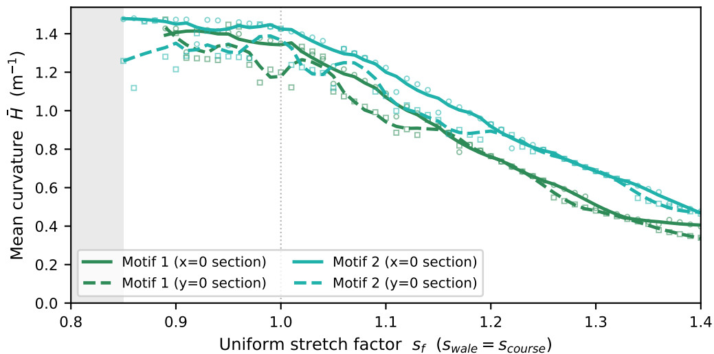
Section curvature vs uniform s_f (markers = individual runs, lines = Savitzky-Golay trend)
