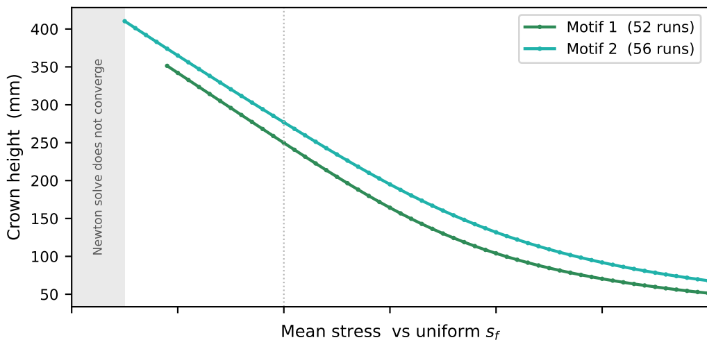
Crown height vs uniform s_f
