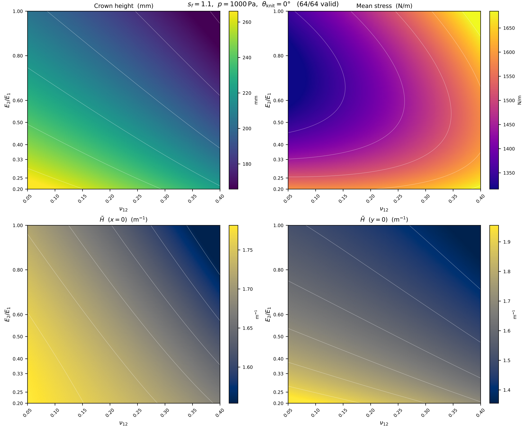
Fig T — E_2/E_1 \times \nu_{12} response surfaces ( E_1 = 7000 \text{ N/m} )
