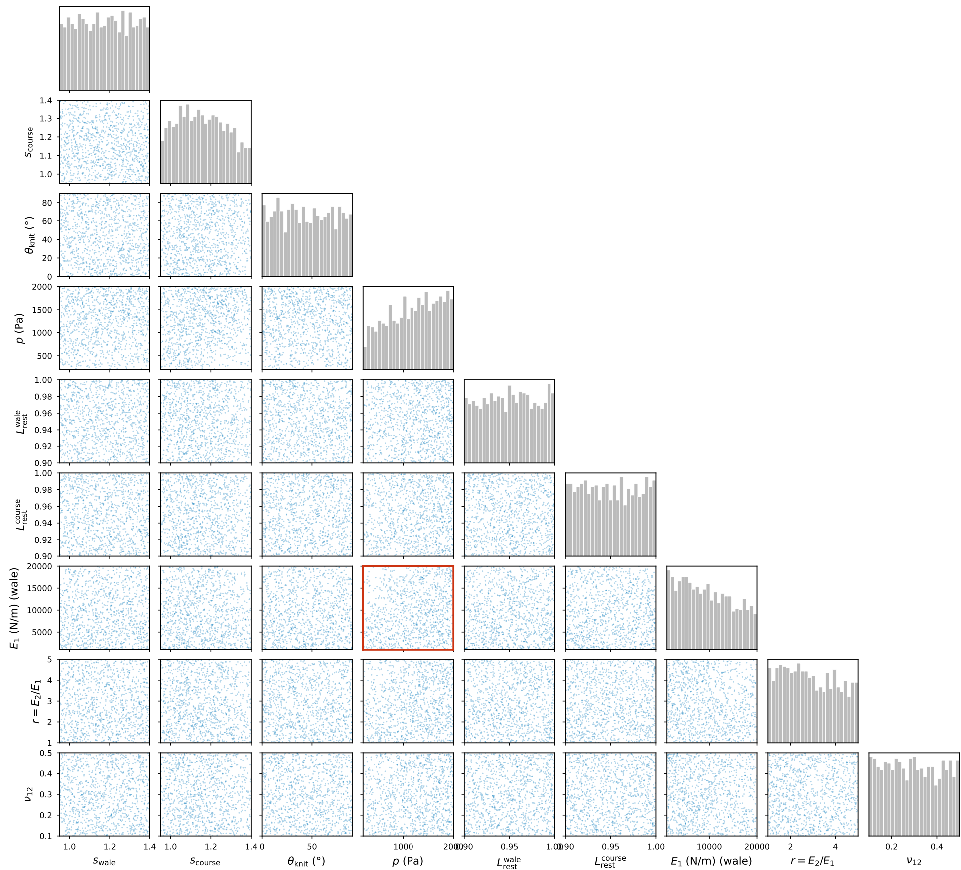
Training design coverage — cable, validity box, s \geq 0.95 (9-D, 1024 runs of 1356 planned, 76% retained) largest pairwise |r| = 0.168 (pressure, E1), outlined in red
