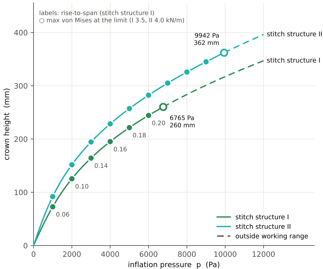
(a) crown height against pressure, s_{wale} = 1.1 , s_{course} = 1.1
