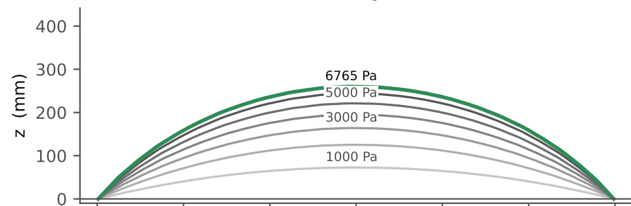
(b) stitch structure I, section through the crown
