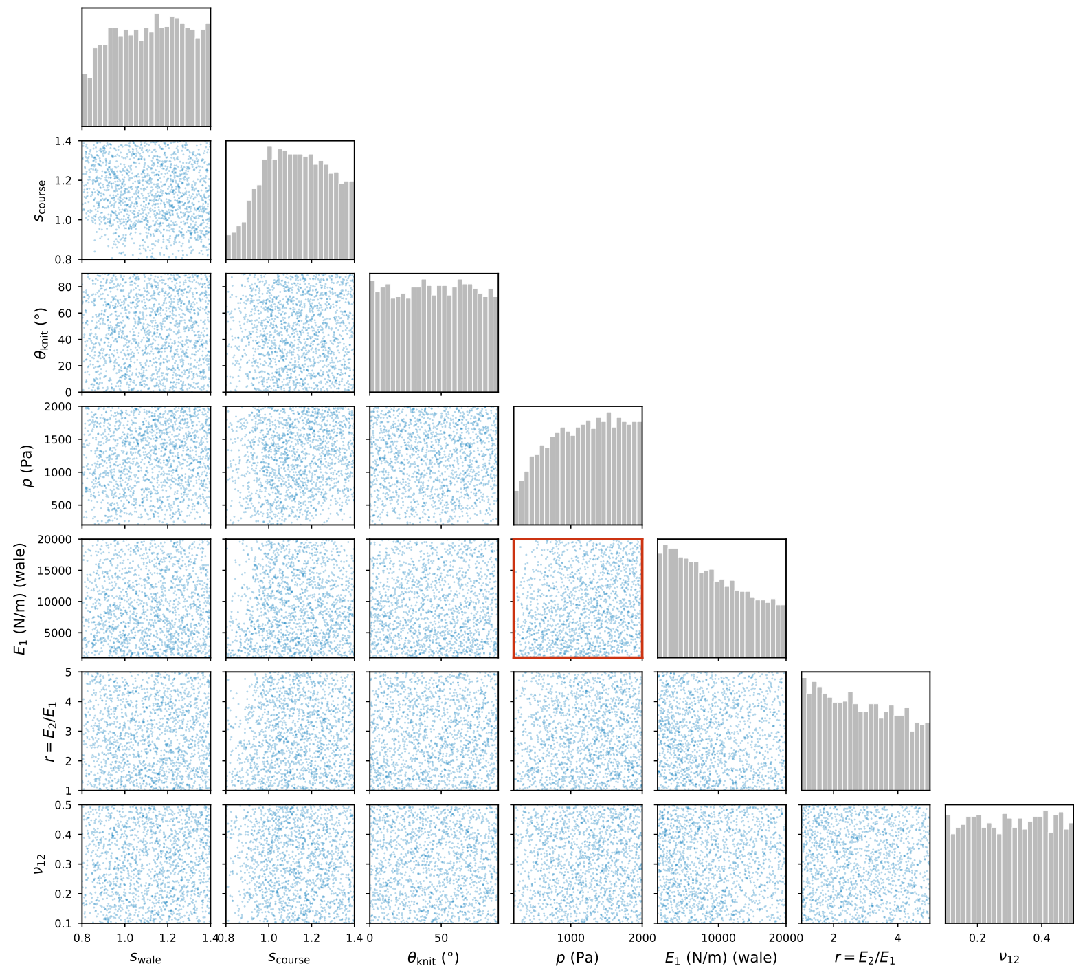
Training design coverage — no cable, full box (7-D, 1618 runs of 2400 planned, 67% retained) largest pairwise |r| = 0.165 (pressure, E1), outlined in red
