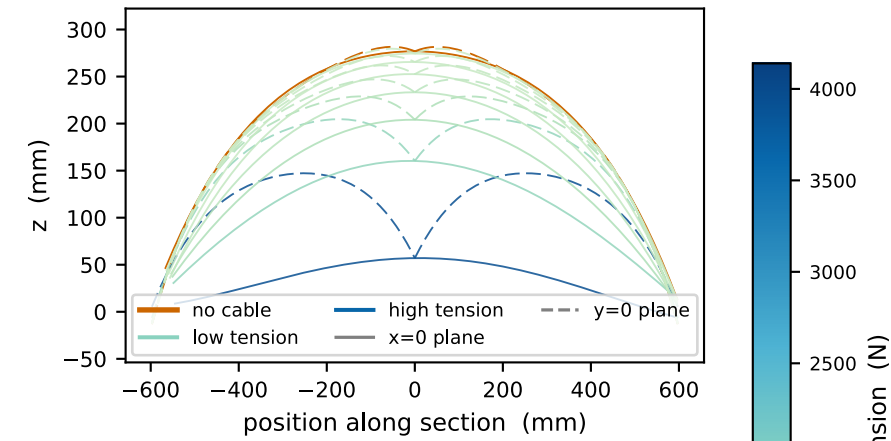
Motif 2 — shape profiles (solid= x=0 , dashed= y=0 )
