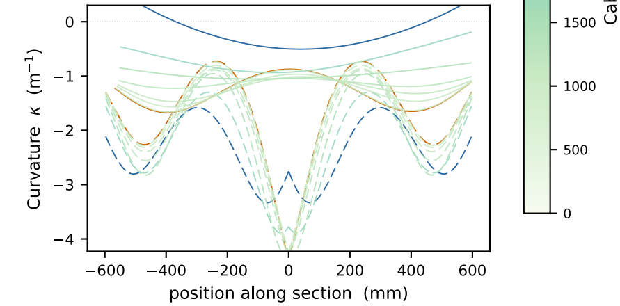
Motif 2 — section curvature (solid= x=0 , dashed= y=0 )
