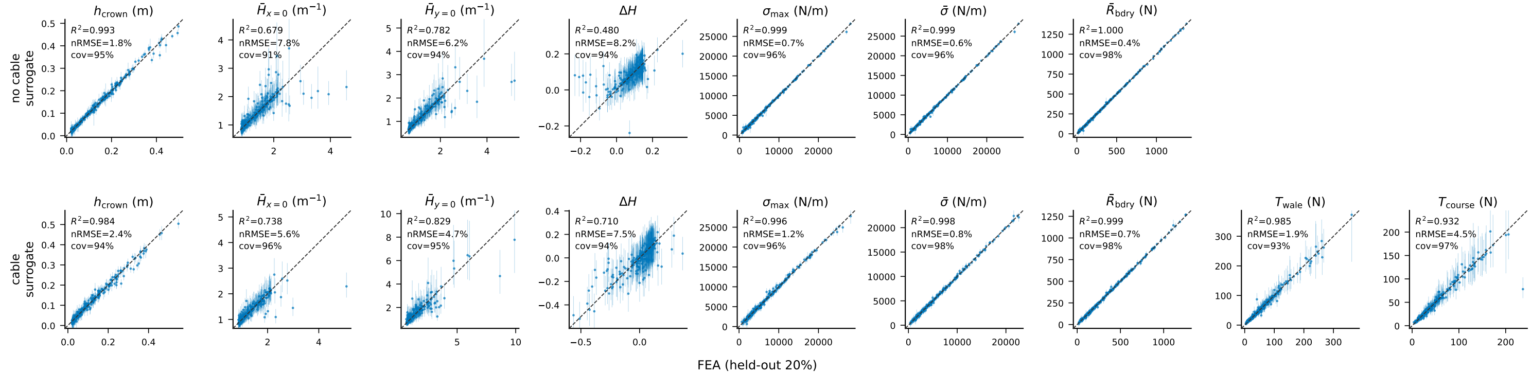
Surrogate accuracy on held-out runs: prediction vs FEA, with 95% predictive intervals (full box)
