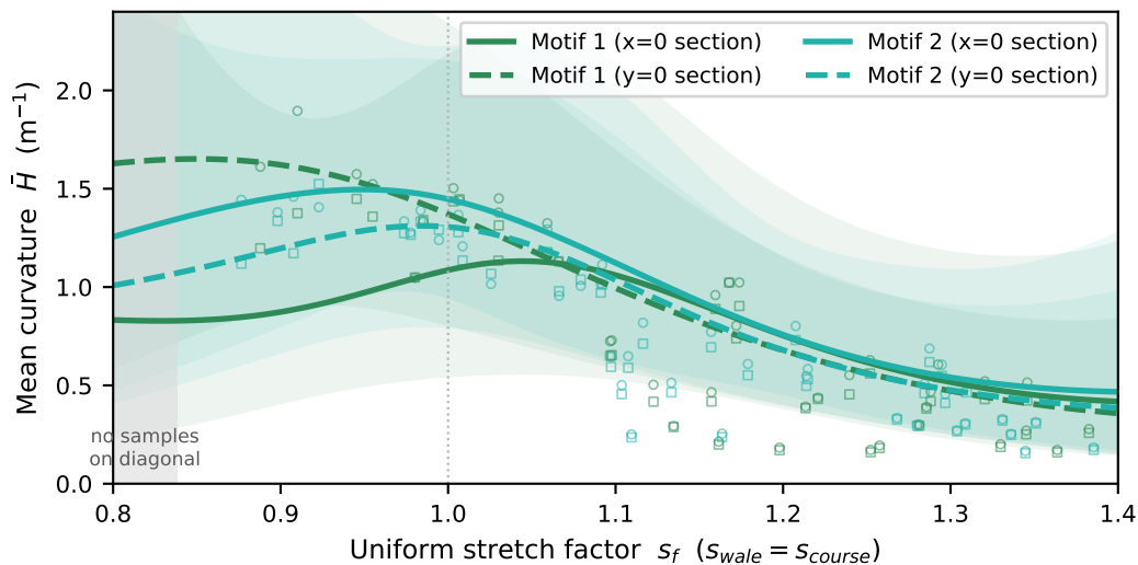
Section curvature vs uniform s_f (log-space GP, band = \pm 2\sigma , markers = quasi-isotropic samples)
