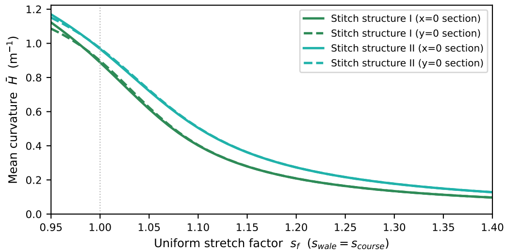
Section curvature vs uniform s_f (Savitzky-Golay trend through one FEA run per s_f )
