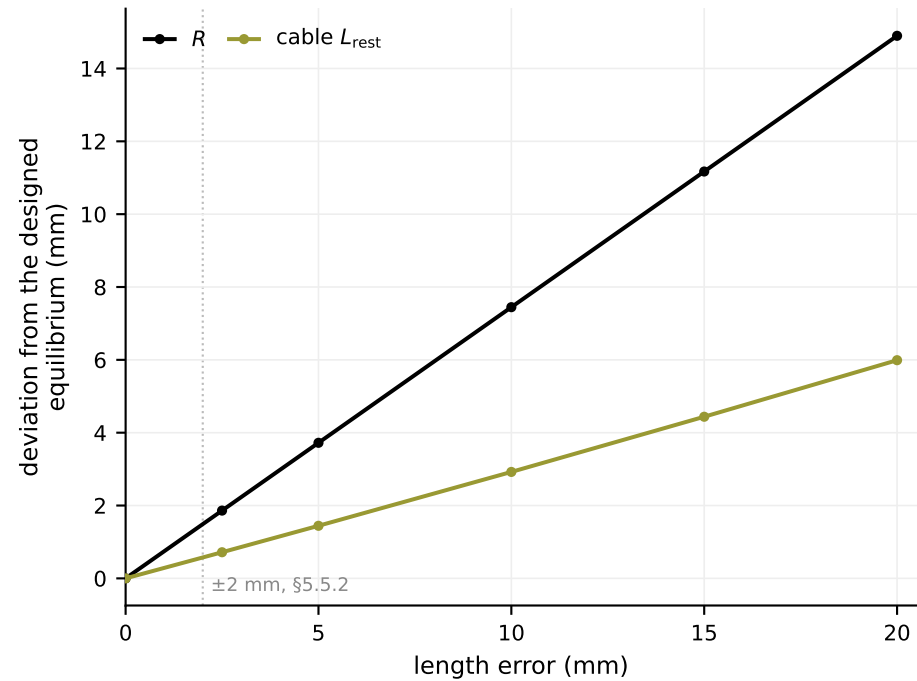
(e) creased shell: boundary radius and cable rest length
