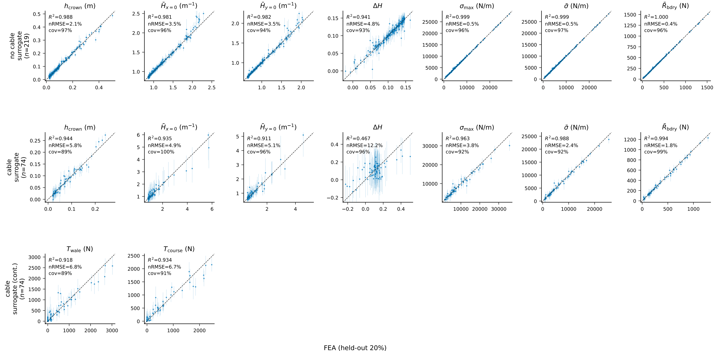
Surrogate accuracy on held-out runs: prediction vs FEA, with 95% predictive intervals (validity box, s \geq 0.95 )
