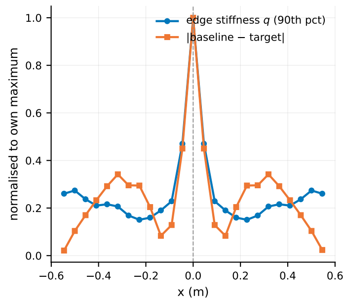
(c) the stiff line and the mismatch are the same line
