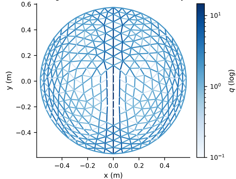
(a) FDM force density q per edge the target was form-found with a valley tie
