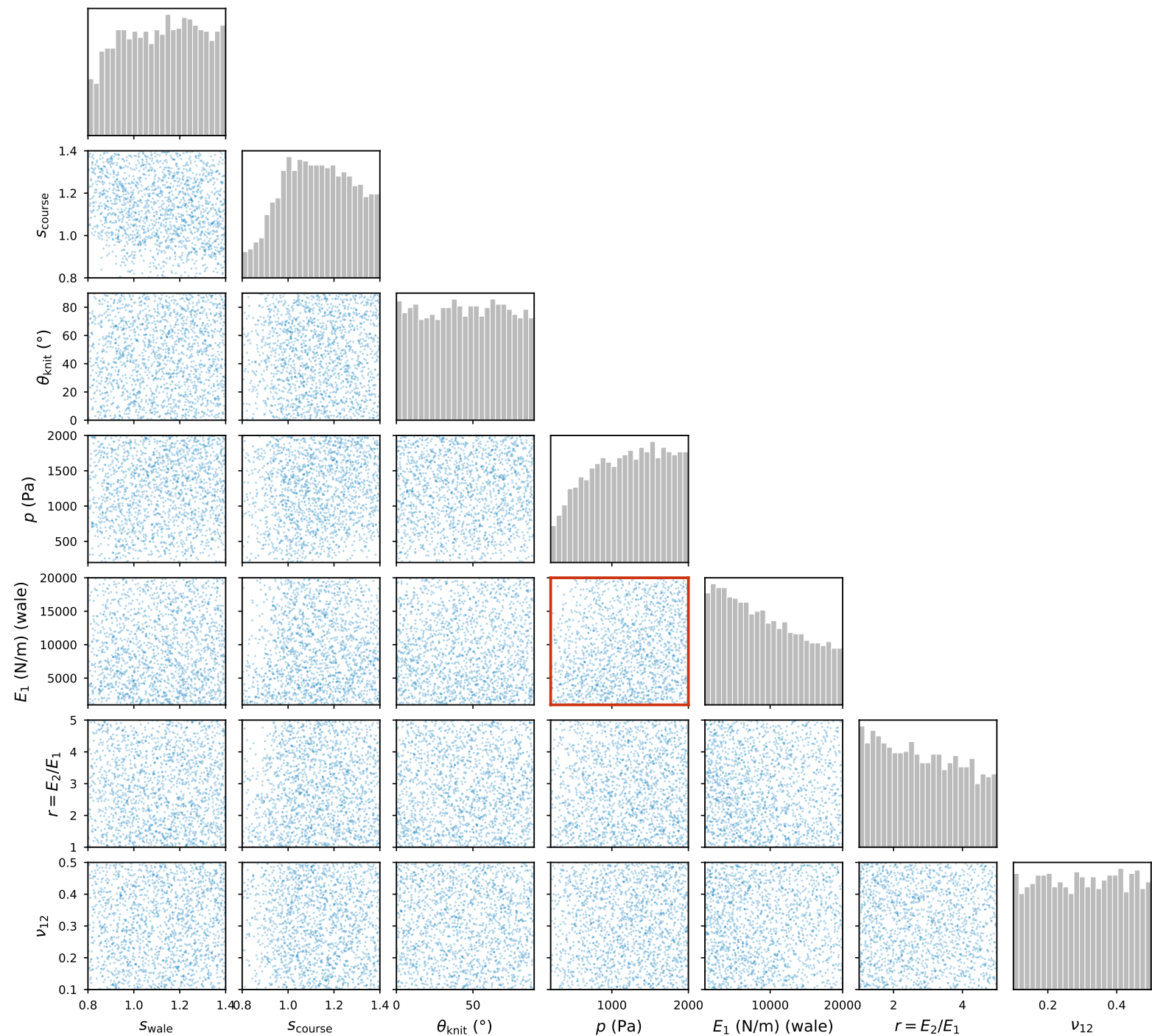
Training design coverage — no cable (7-D, 1618 runs of 2400 planned, 67% retained) largest pairwise |r| = 0.165 (pressure, E1), outlined in red
