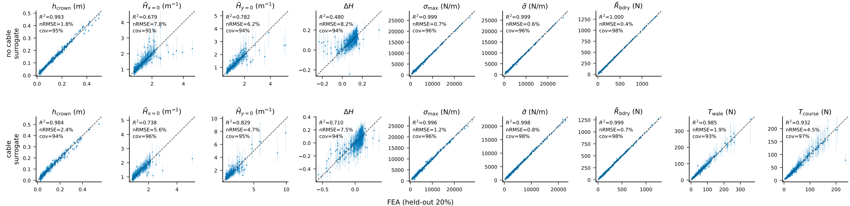
Surrogate accuracy on held-out runs: prediction vs FEA, with 95% predictive intervals
