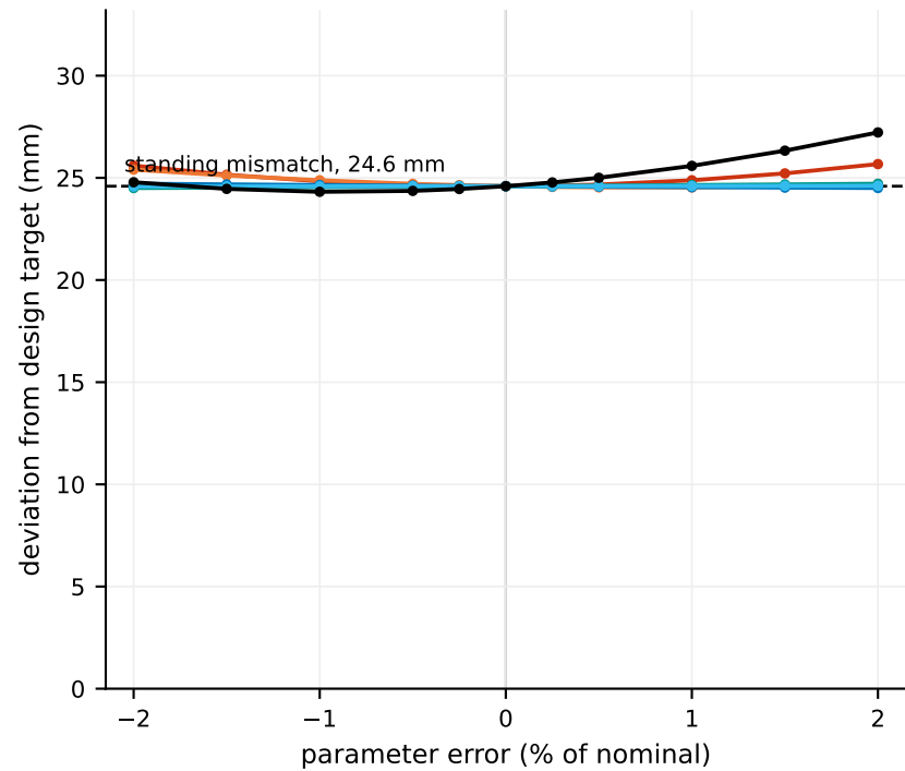
(c) creased shell: deviation from the design target
