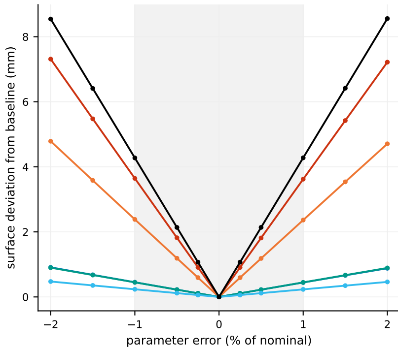
(b) creased shell: how far the surface moves
