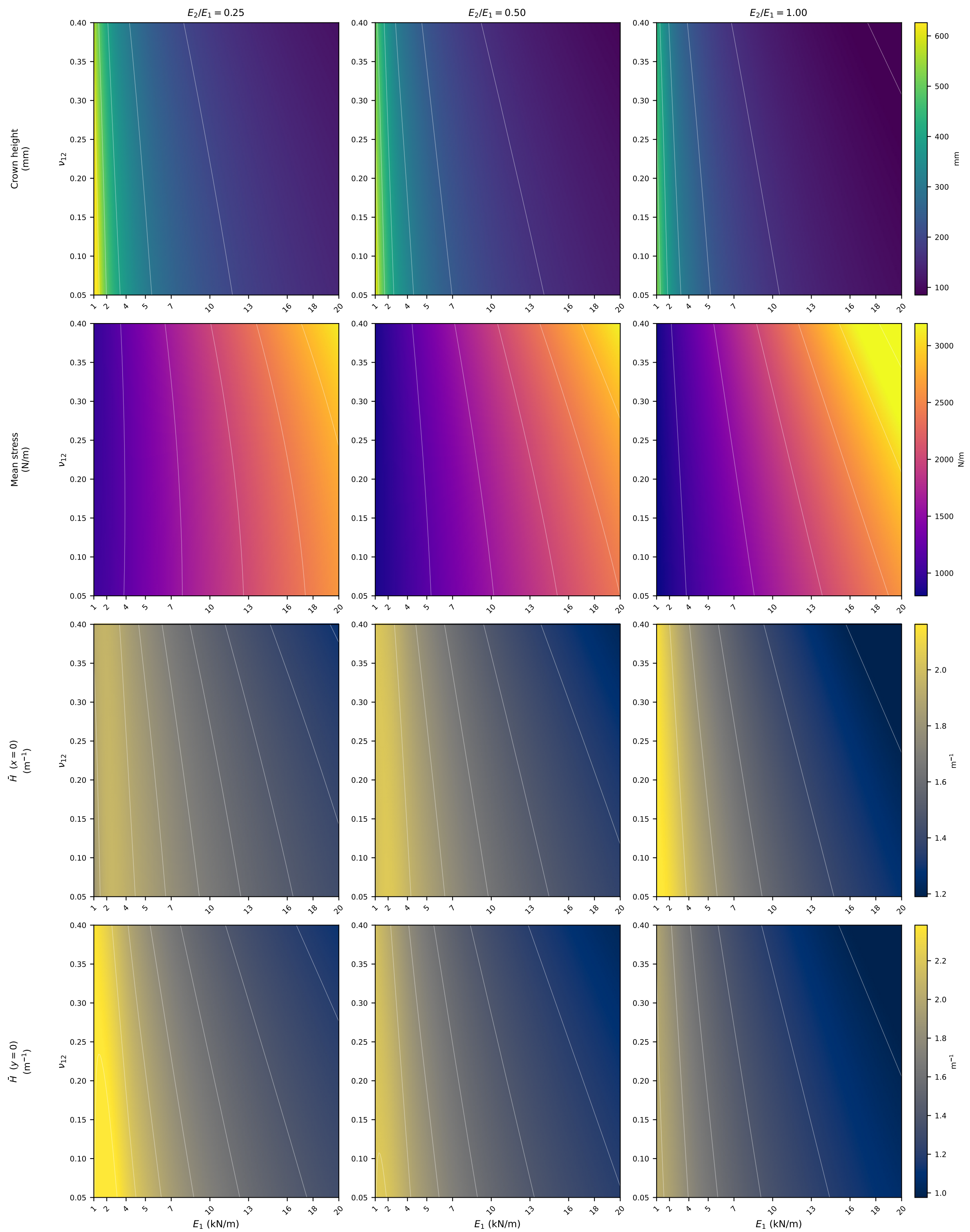
Fig S — E_1 \times v_{12} response surfaces (3 anisotropy slices) s_f = 1.1 , p = 1000 Pa, \theta_{\text{knit}} = 0^\circ
