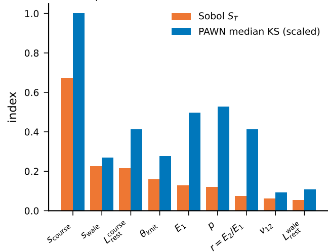
(c) cable \Delta H : variance-based vs moment-independent Spearman rank correlation 0.47
