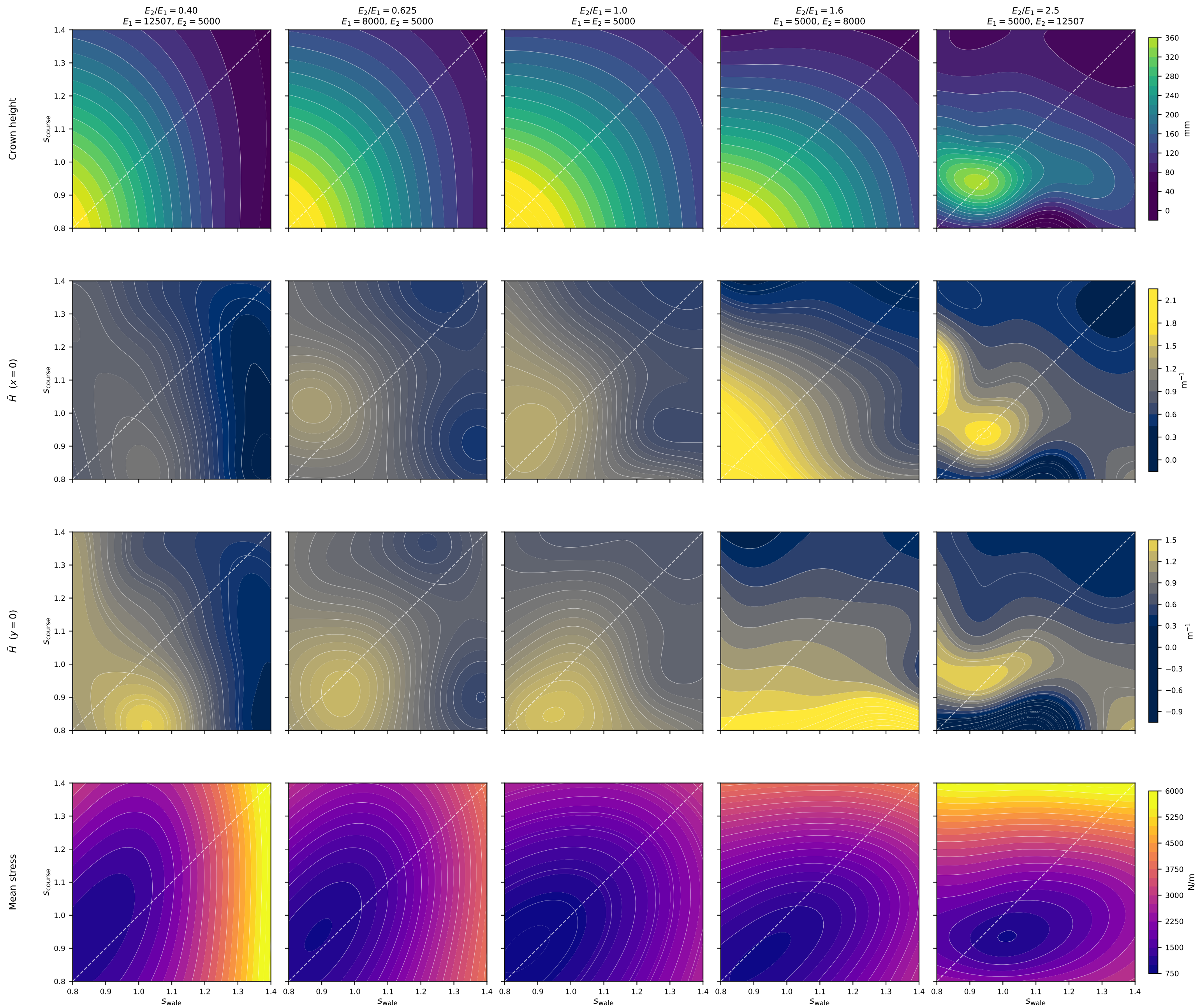
Response surfaces: s_{\text{wale}} \times s_{\text{course}} across E_1/E_2 anisotropy ( \theta_{\text{knit}} = 0^\circ , p = 1000 \text{ Pa} ; dashed = uniform s_f )
