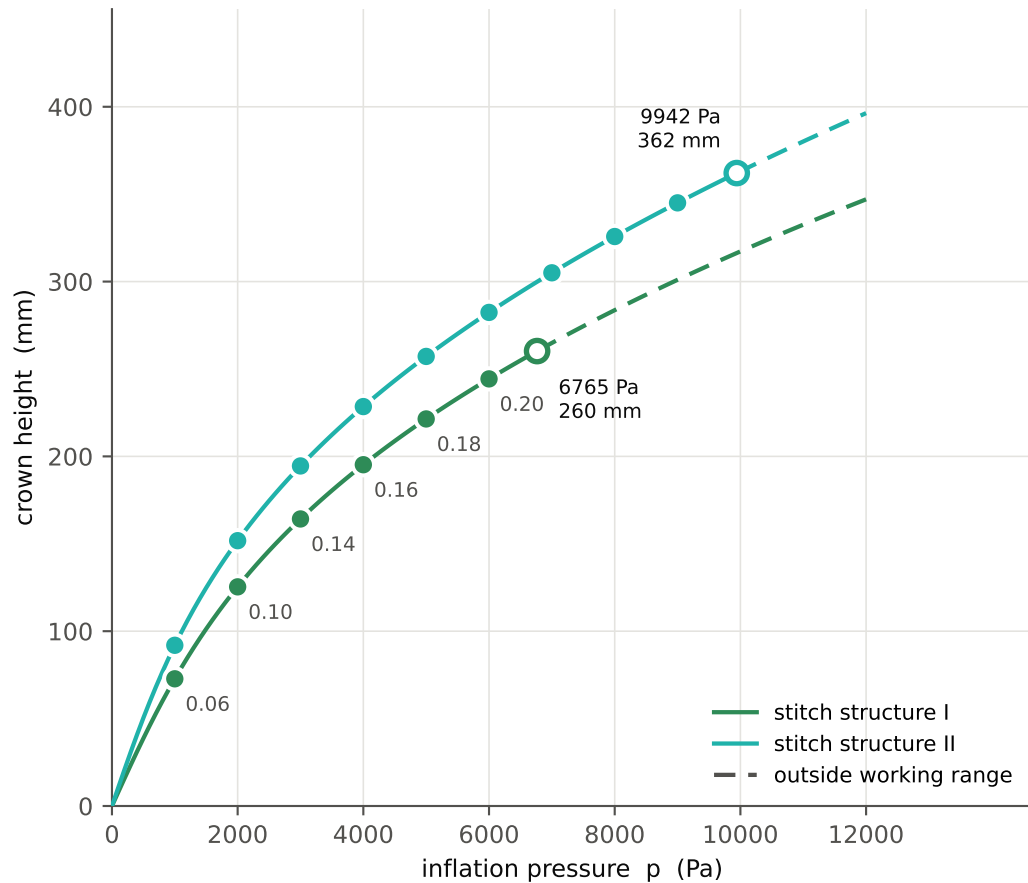
(a) crown height against pressure, s_{wale} = 1.1 , s_{course} = 1.1
