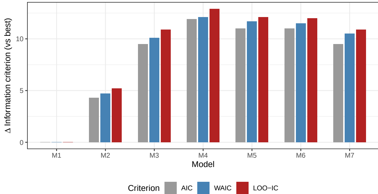
Model comparison: frequentist AIC vs Bayesian WAIC and LOO-IC
