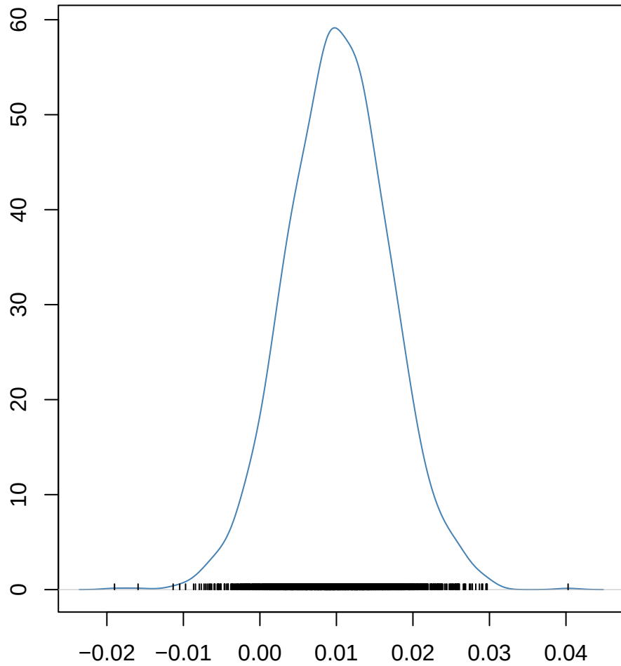
logTotGenes_raw~flight
