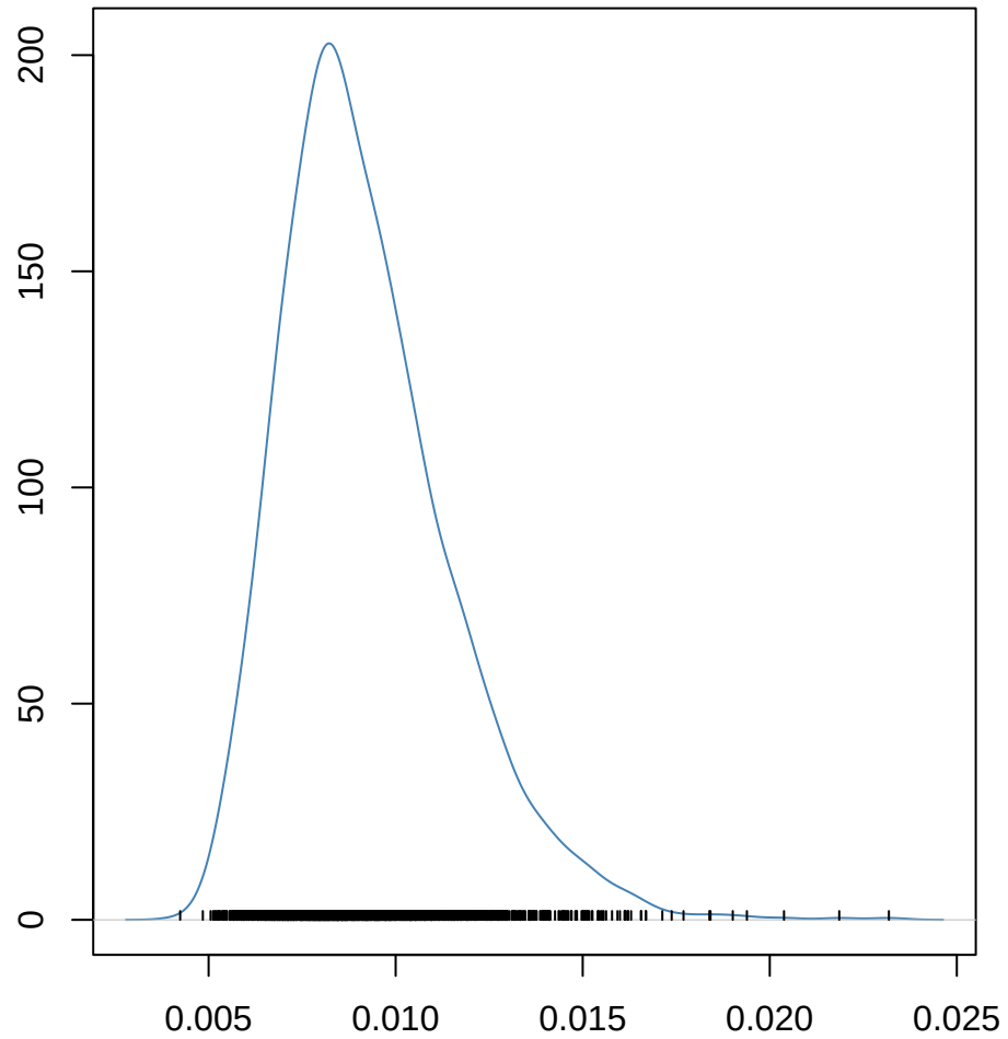
propAccelDn~~propAccelDn
