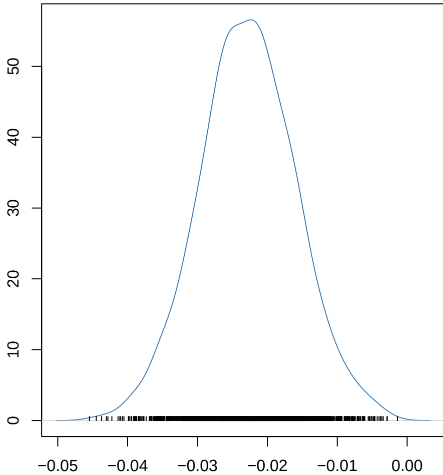
propAccelDn~flight
