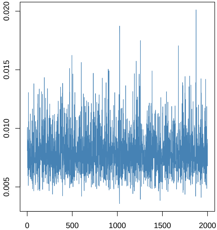
logTotGenes_raw~~logTotGenes_raw
