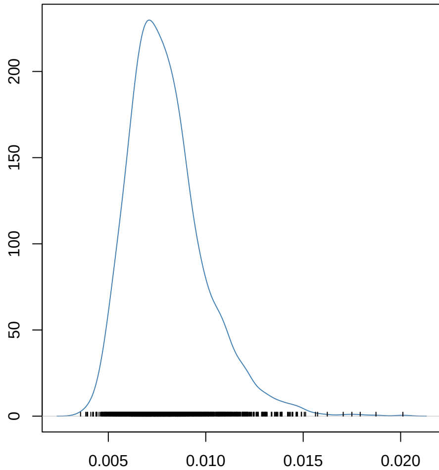
logTotGenes_raw~~logTotGenes_raw
