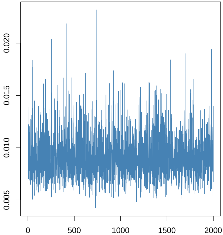
propAccelDn~~propAccelDn
