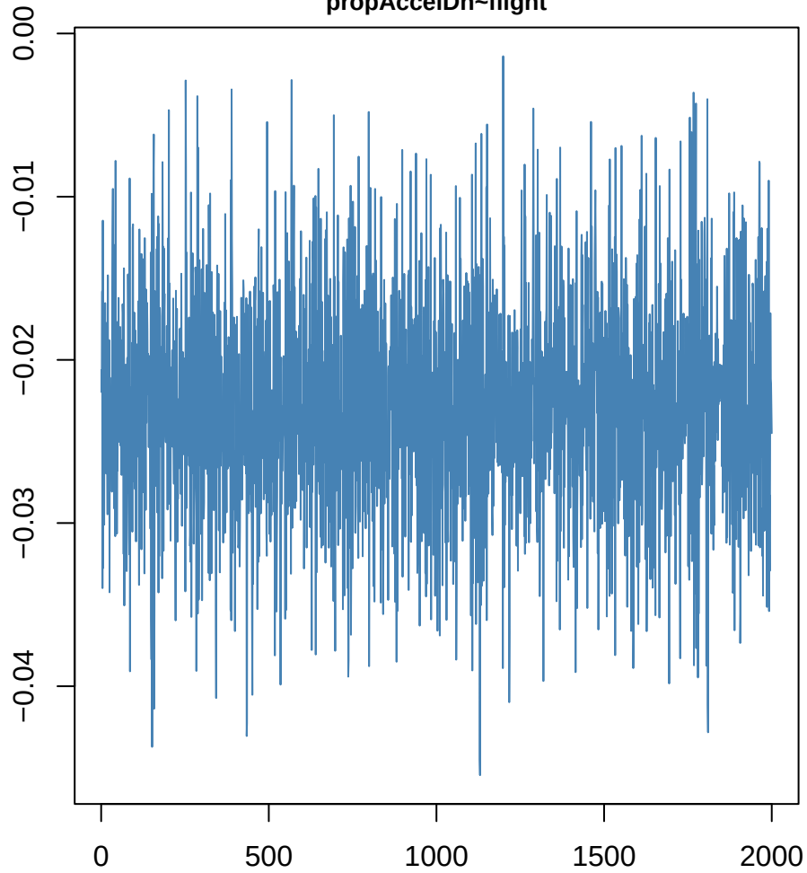
propAccelDn~flight
