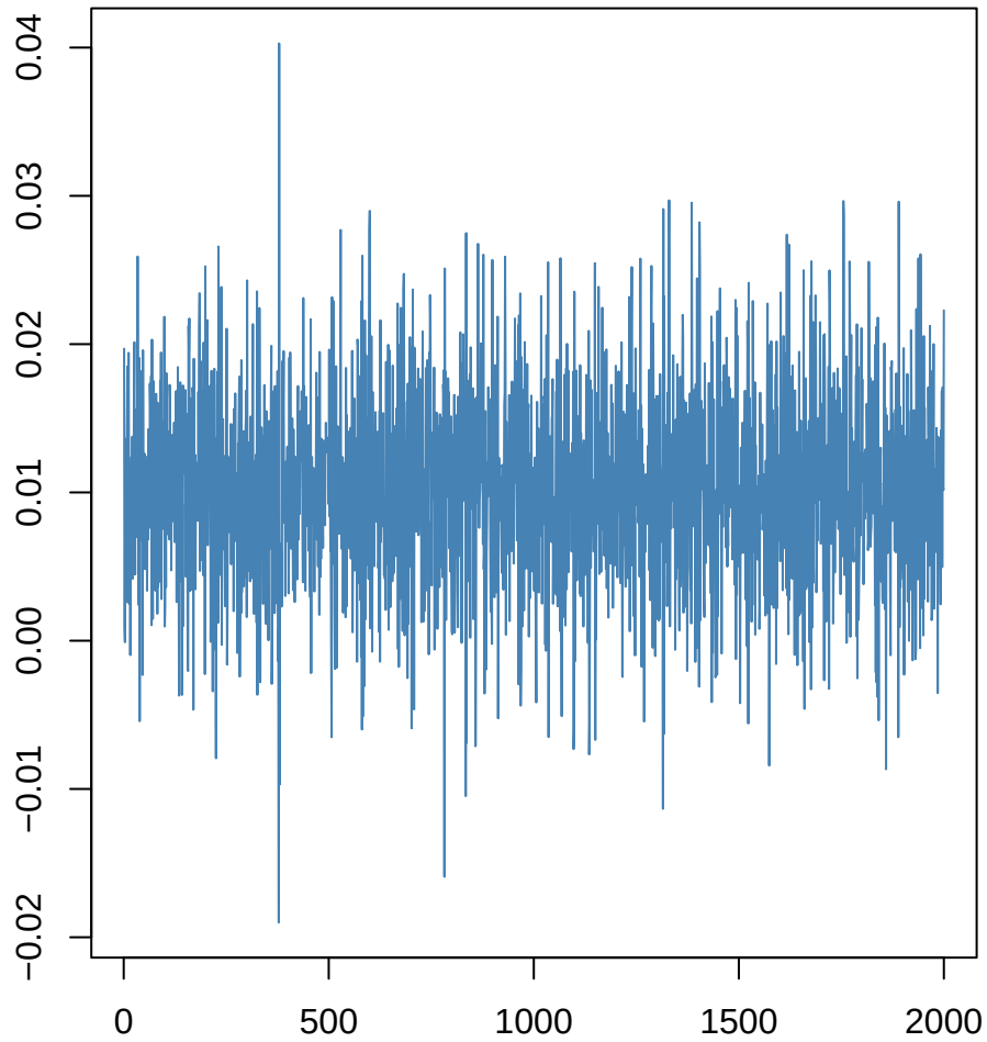
logTotGenes_raw~flight
