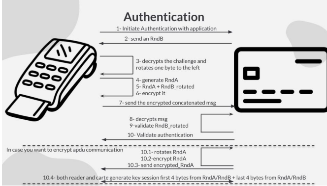
Fig. 5. Authentication process
