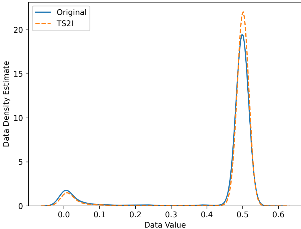
network_traffic
