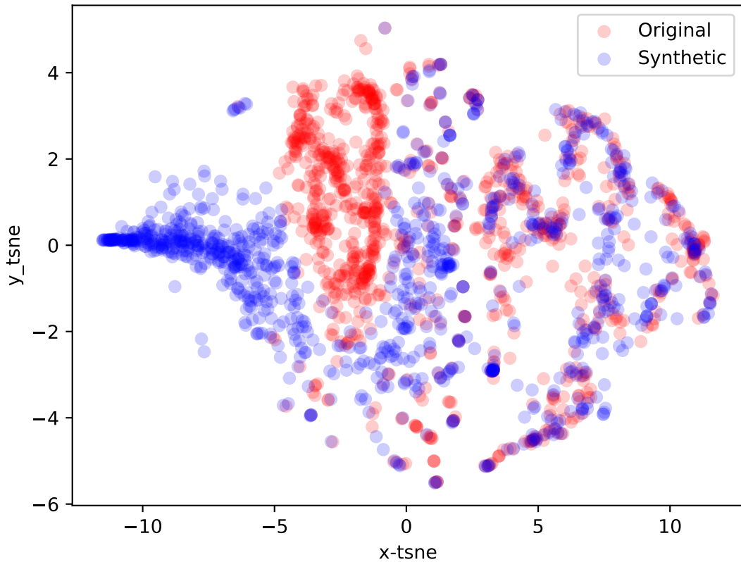
t-SNE plot
