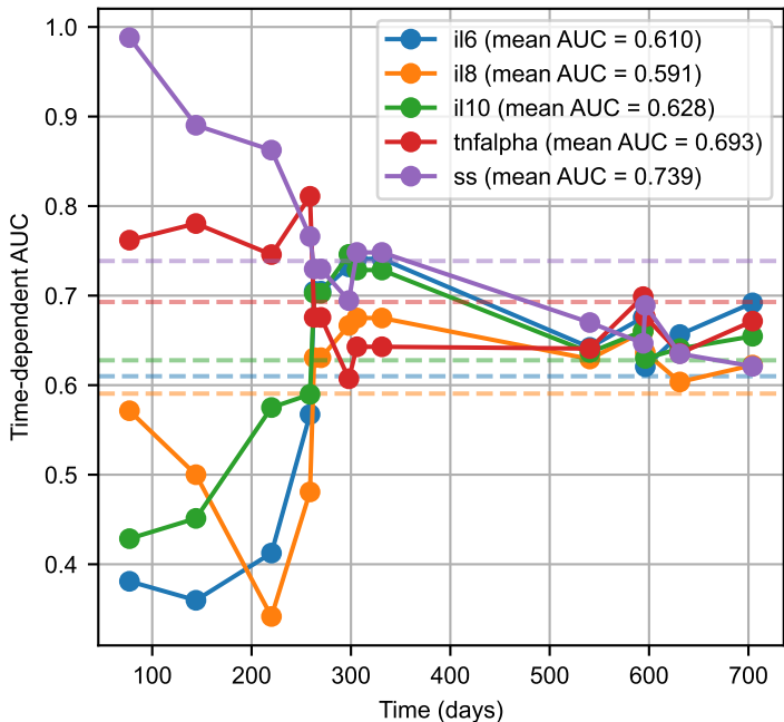
Individual feature AUC curves
