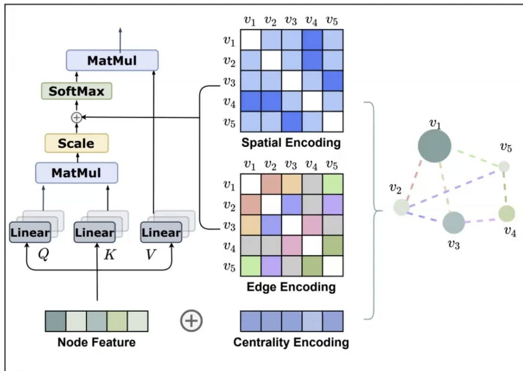
Extending Transformers to encode Graph Edges
