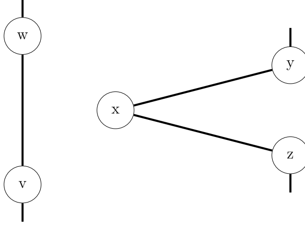
Figure 5: Starting point of the local search step. We denote the left hamiltonian path that contains the vertices v and w as H_i , the right one with H_j .
