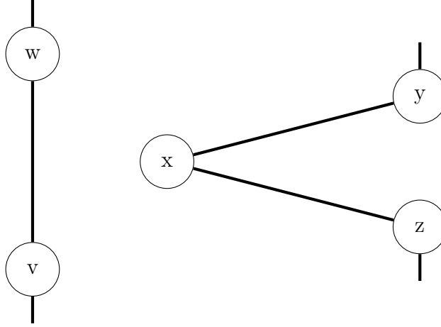
Figure 5: Starting point of the local search step. We denote the left hamiltonian path that contains the vertices v and w as H_i .
