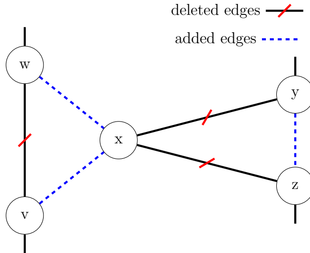
Figure 6: Moving x \in V(H_j) requires deletion and creating edges in both hamiltonian paths H_i and H_j .
