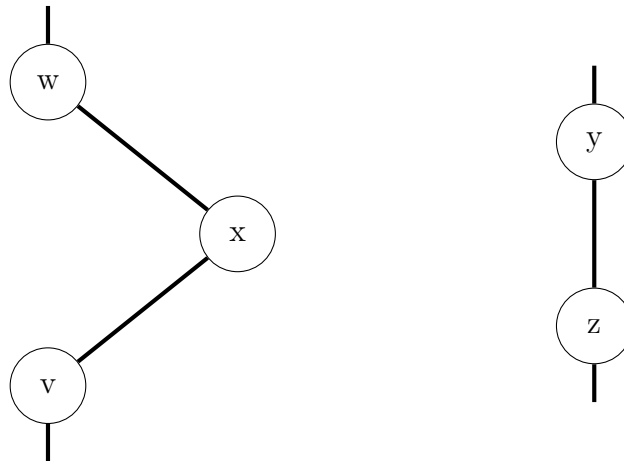
Figure 7: After moving vertex x \in V(H_j) to hamiltonian path H_i .
