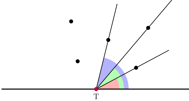
Figure 3: Sort heliostats by computed angles. For K \in \mathbb{N} partitions we obtain \left\lceil \frac{|V_H|}{K} \right\rceil heliostats in each partition.
