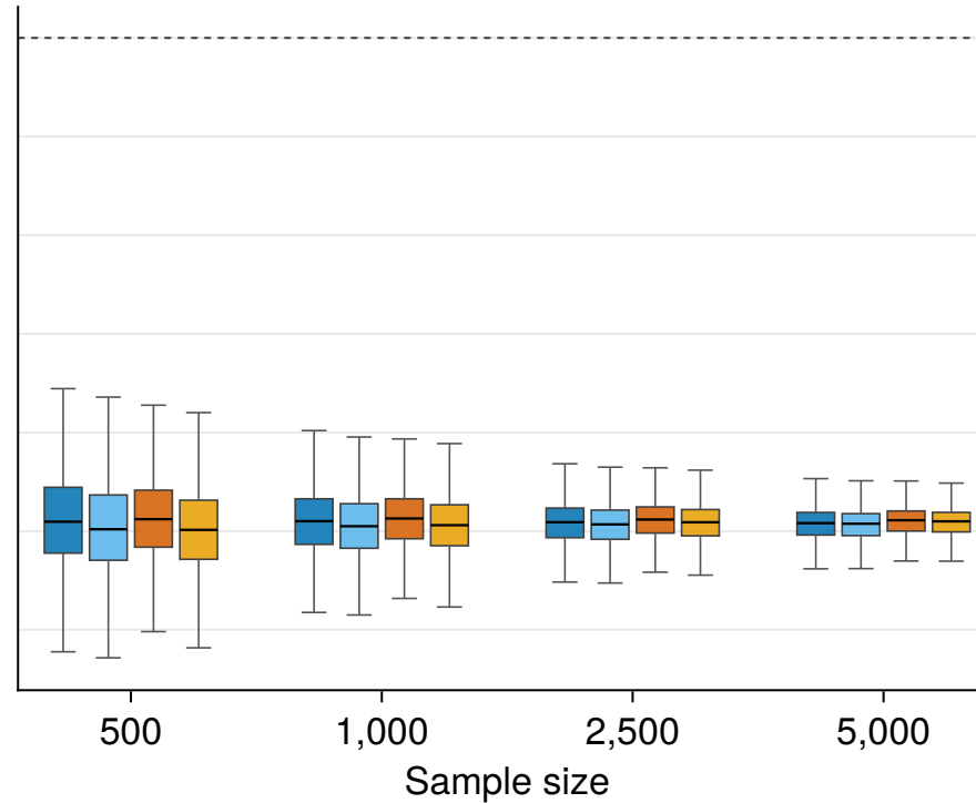
Student t_8
