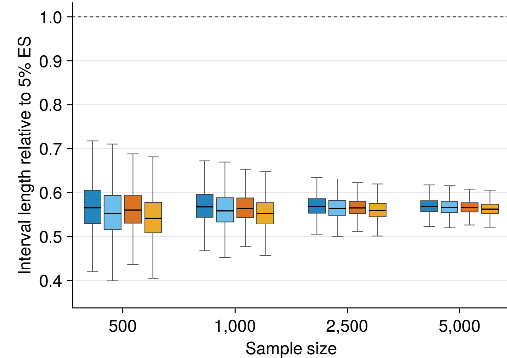
Normal
