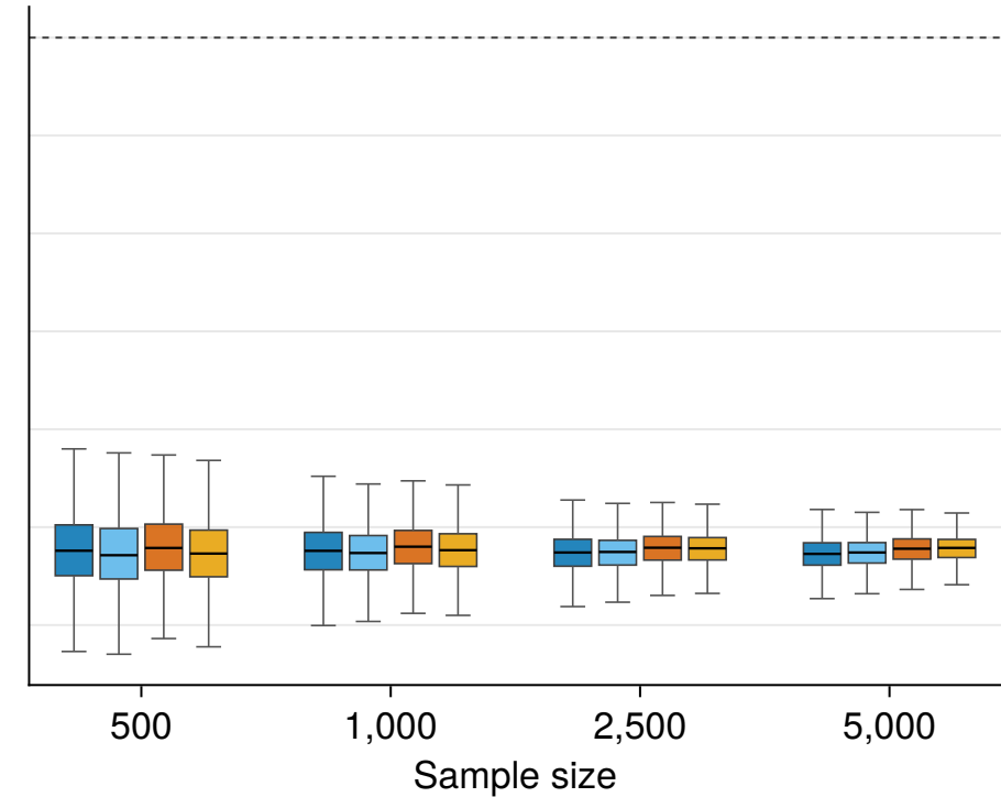
Student t_4
