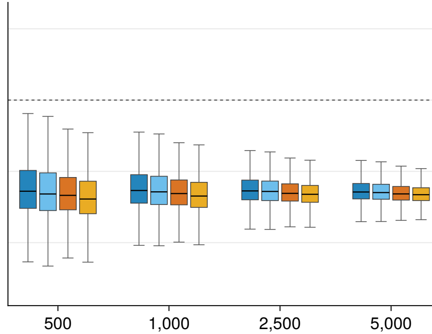
Student t_8
