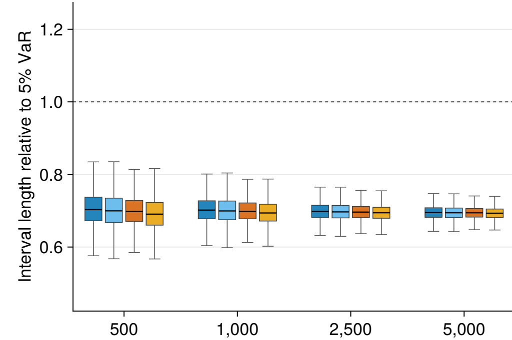
Normal
