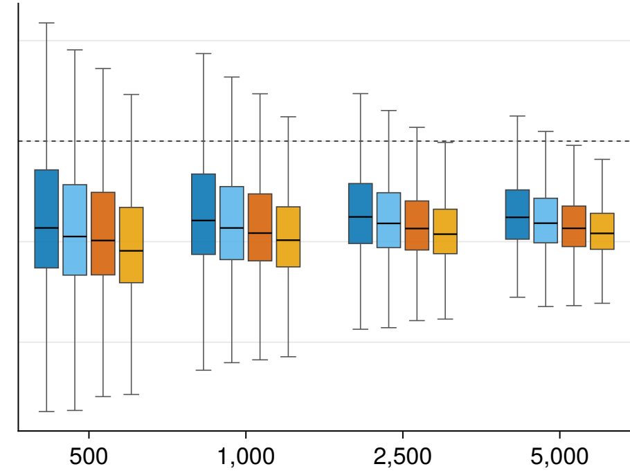
Student t_4
