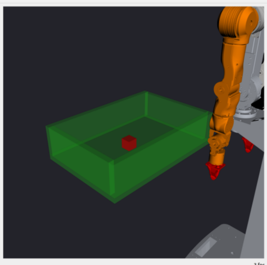
(c) Locked — Pitch target: IK failure
