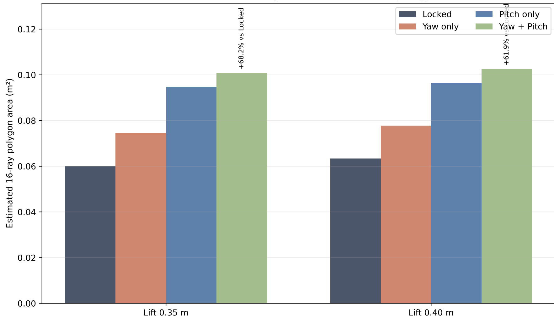
Planning-only 16-ray polygon area estimate (not exact continuous workspace; increase is not a synergy claim)
