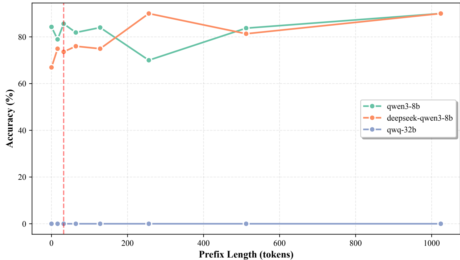
Oracle Prefix: Accuracy vs Prefix Length
