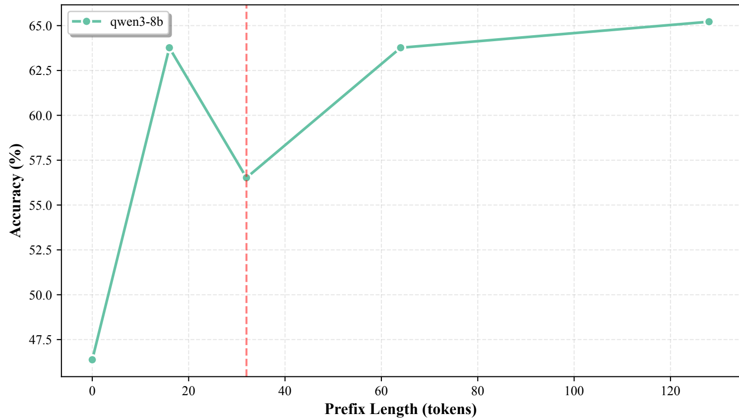
Self-Correct Prefix: Accuracy vs Prefix Length
