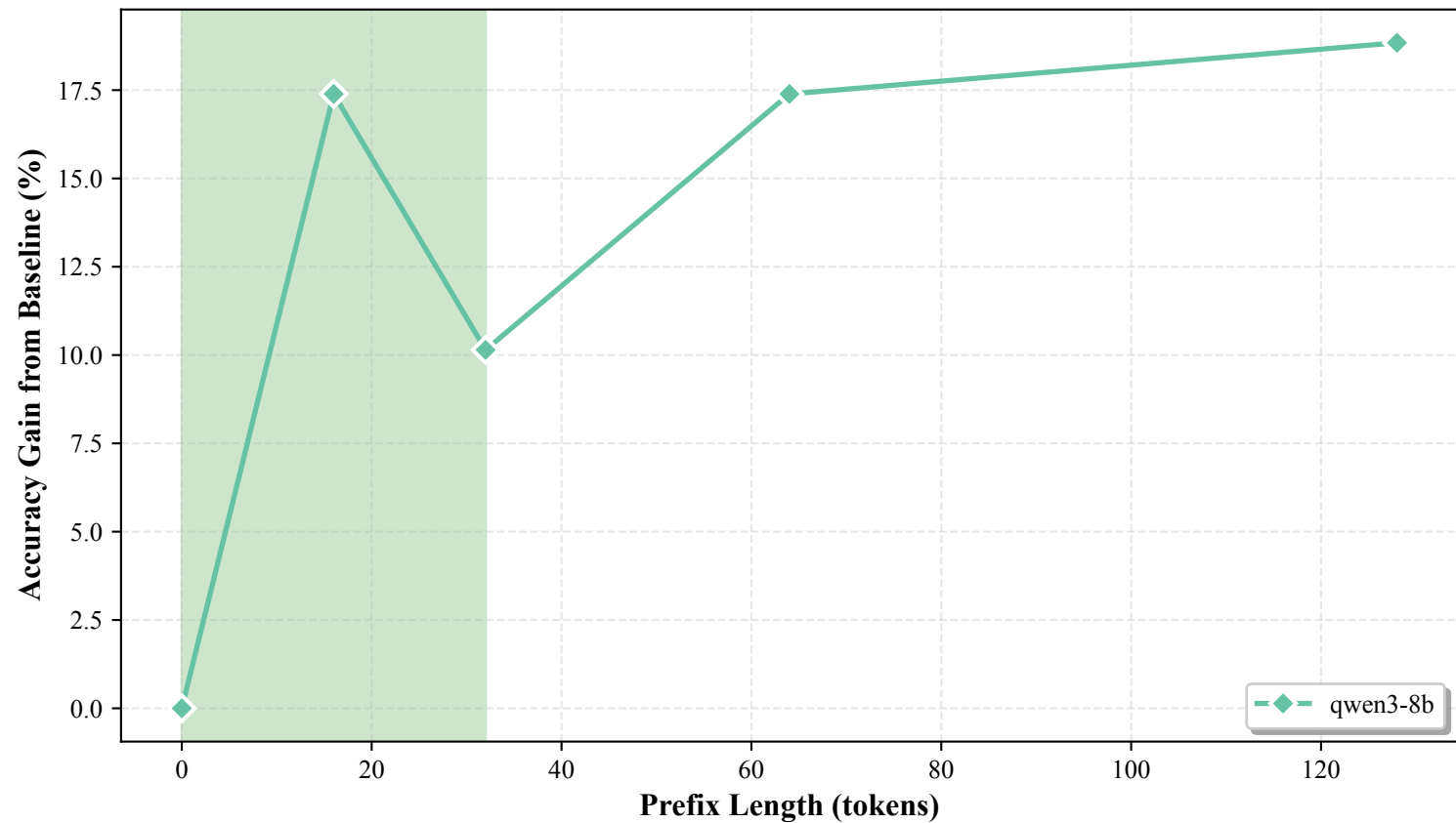
Self-Correct Prefix: Cumulative Accuracy Gain
