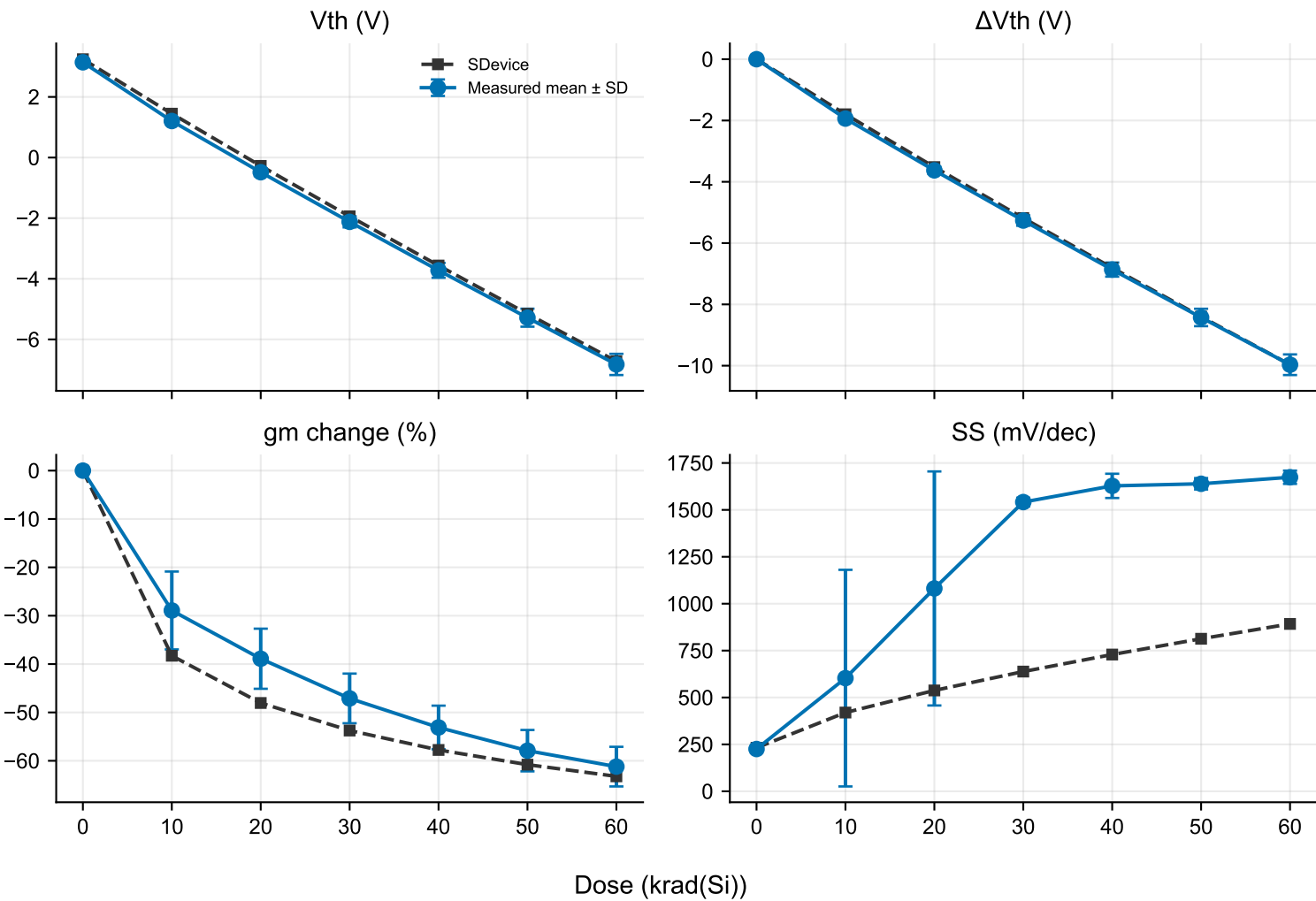
T transfer metrics: measured (n=3) and SDevice
